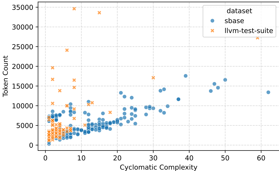
Function Complexity vs. Context Window Size
